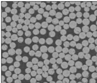
CROSS SECTION x700
